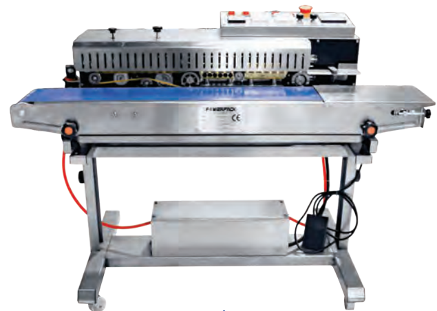
CONTINUOUS BAND SEALER W/ VACUUM NITROGEN FILLING
